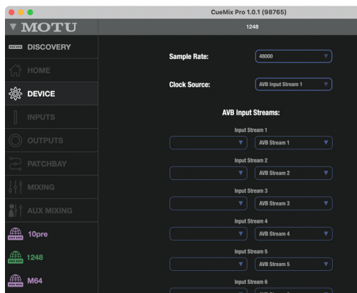
Figure 6-12: A MOTU 1248 selected in the sidebar. Basic network-related settings are available in the Device tab.
